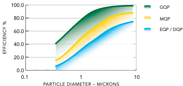
COMPOSITE MINIMUM EFFICIENCY CURVE
